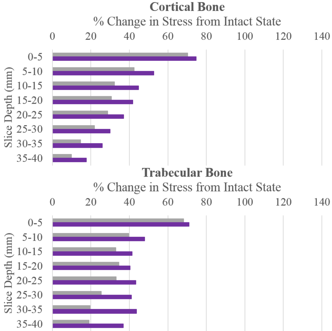
Figure E-2: Changes in Proximal Bone Stress with a Large Collared Implant at 75° Abduction
