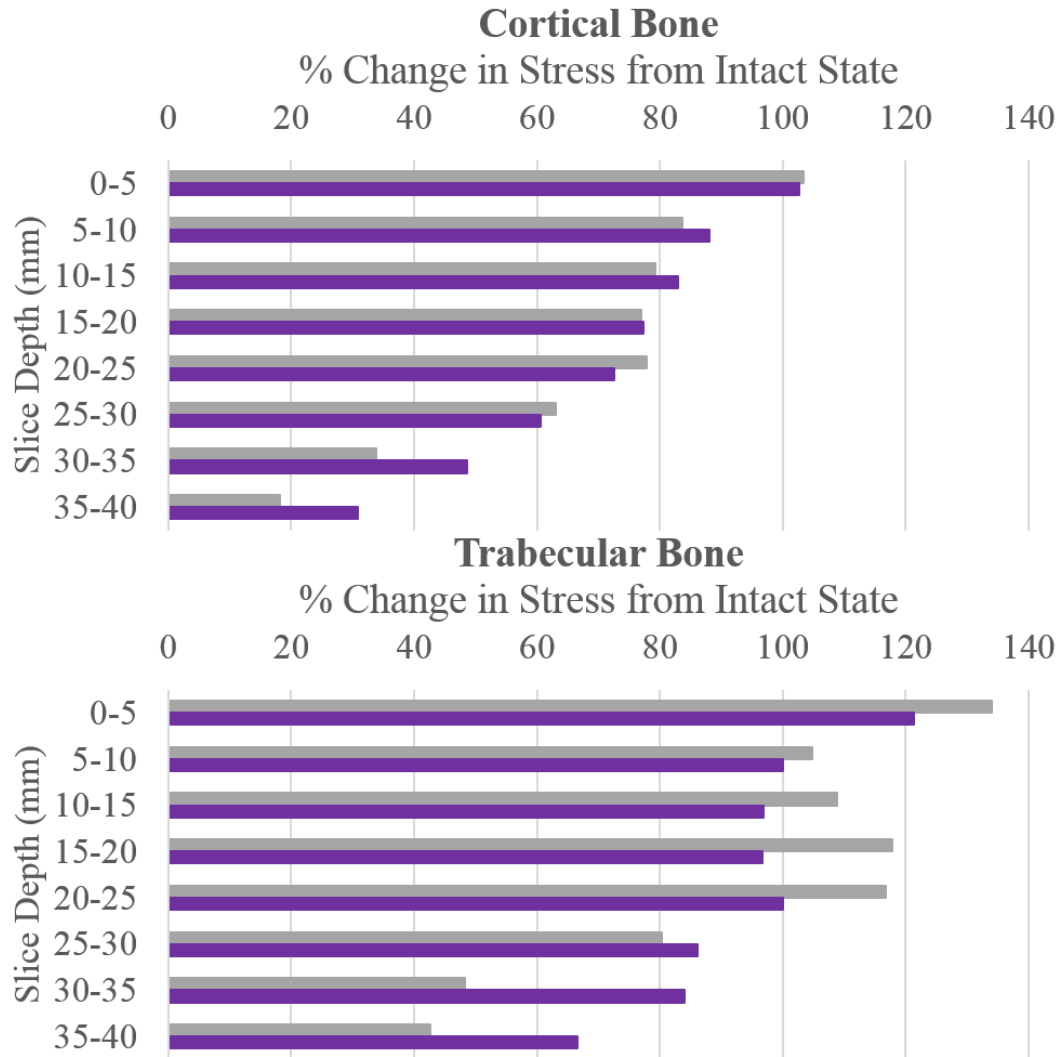
Figure E-3: Changes in Proximal Bone Stress with a Large Collarless Implant at 75° Abduction
