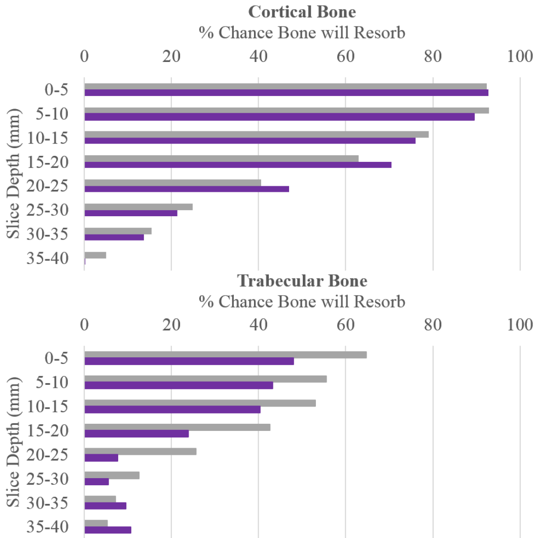
Figure E-5: Changes in Percent Volume of Bone Expected to Resorb with a Large Collarless Implant at 75° Abduction
