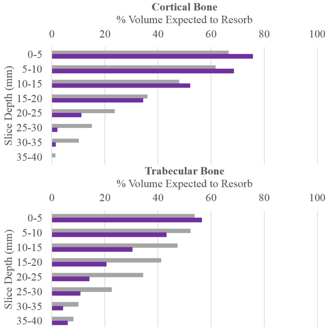
Figure E-4: Changes in Percent Volume of Bone Expected to Resorb with a Large Collared Implant at 75° Abduction
